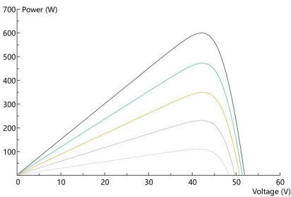
Power-Voltage Curve (600W)
